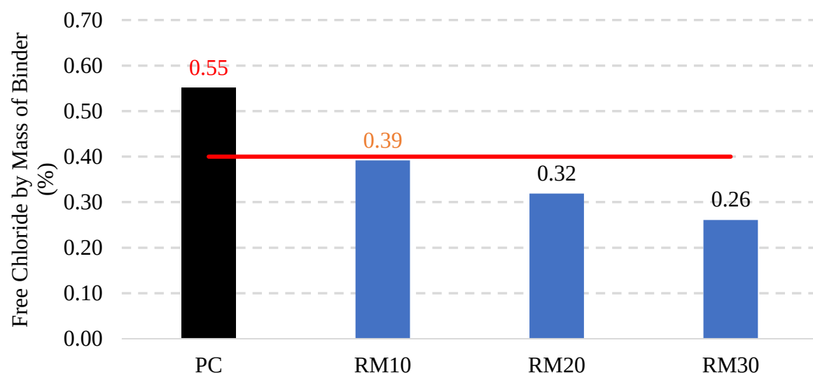
Figure 6. Free Chloride Percent by Mass of Binder for the Red Mud System
