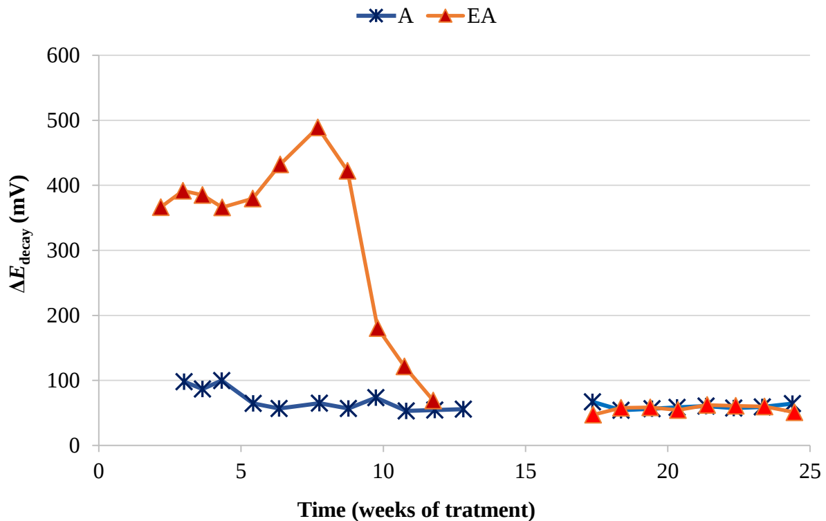
Figure 3. Evolution of \Delta E_{\text{decay}} during the CP treatments. A: CP; EA: ECE + CP. All of them subjected to \text{Cl}^- contamination during the 24 weeks. The electrochemical treatments were interrupted between week 13 and week 17. Adapted from (Carmona, et al, 2015).
