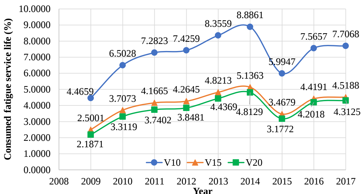
Figure 8. Consumption of longitudinal reinforcement fatigue service life (Own Author, 2019).
