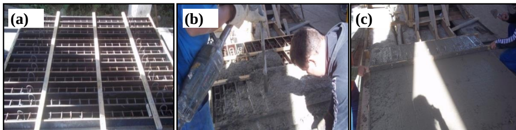
Figure 2. Manufacturing of the reinforced concrete beams – (a) Molds with the reinforcement ready for casting; (b) Casting and vibration; (c) Leveling of the concrete in the molds.
