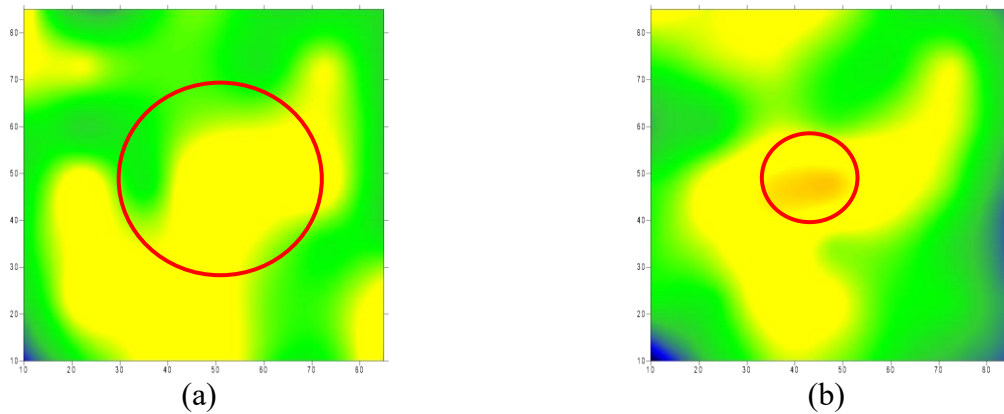
Figure 14. Image corresponding to the depth of: (a) 0,40 m and (b) 0,50 m
