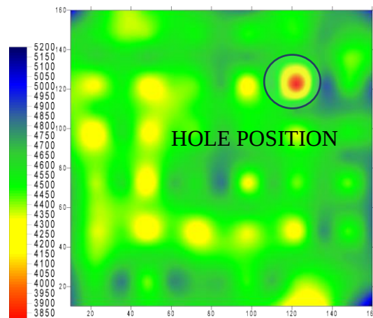
Figure 16. Image corresponding to the depth of 60 cm - full face
