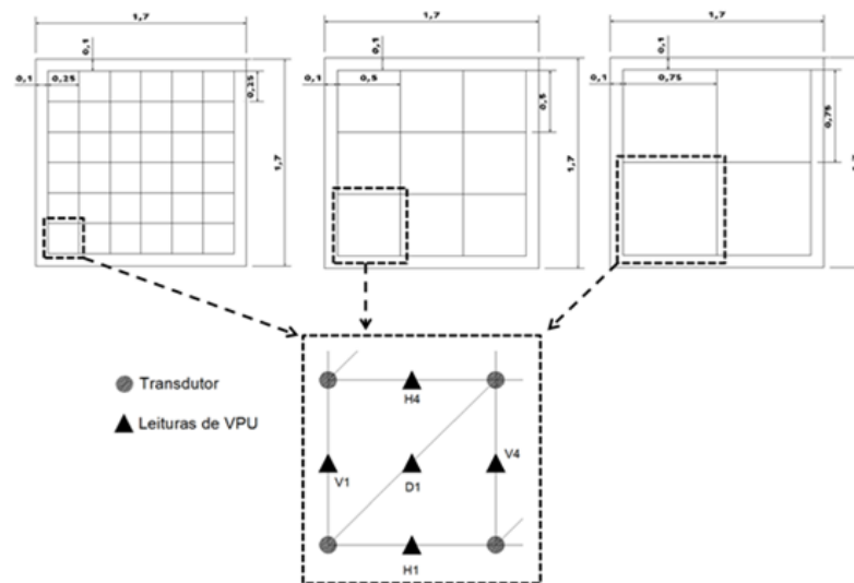
Figure 4. Reading design for each grid
