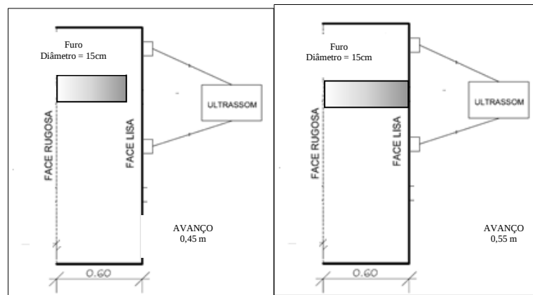
Figure 6. Drill advance diagram
