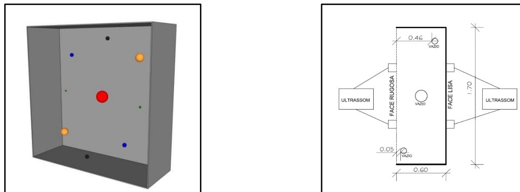
Figure 2. Positioning and depth of voids.
