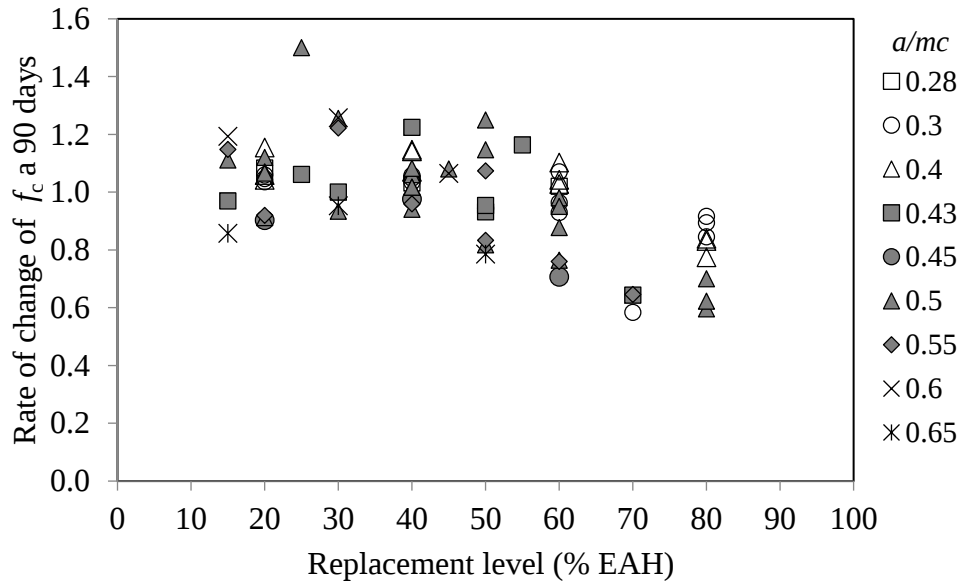
Figure 5. Rate of change (efficiency) of the resistance to real compression f_c of the concretes with slag, at 90 days.
