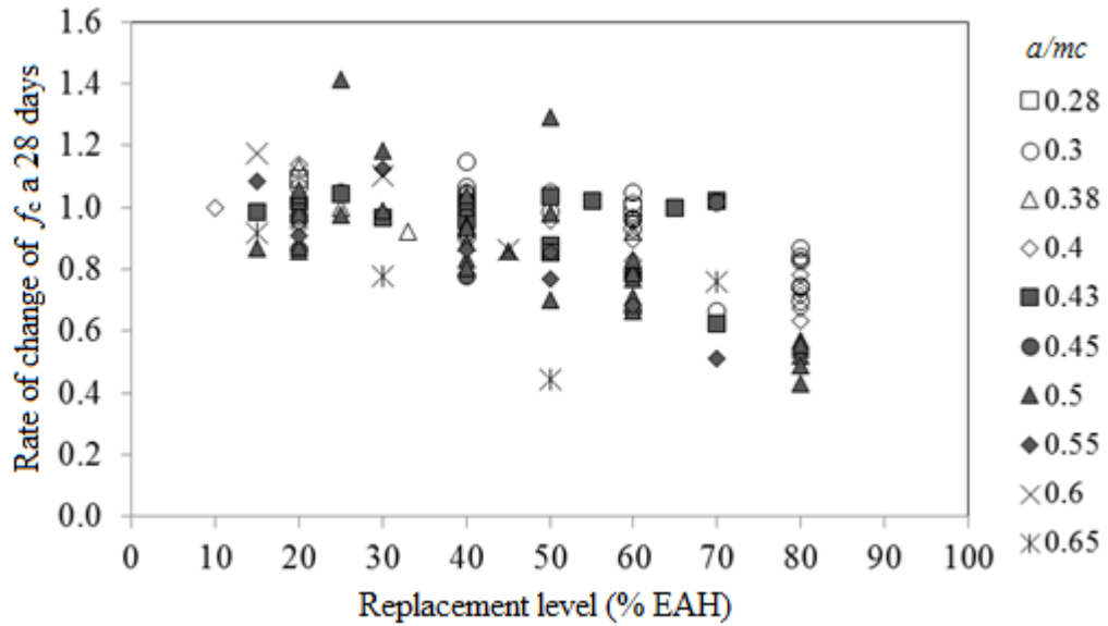
Figure 4. Rate of change (efficiency) of the resistance to real compression f_c of the concretes with slag, at 28 days.
