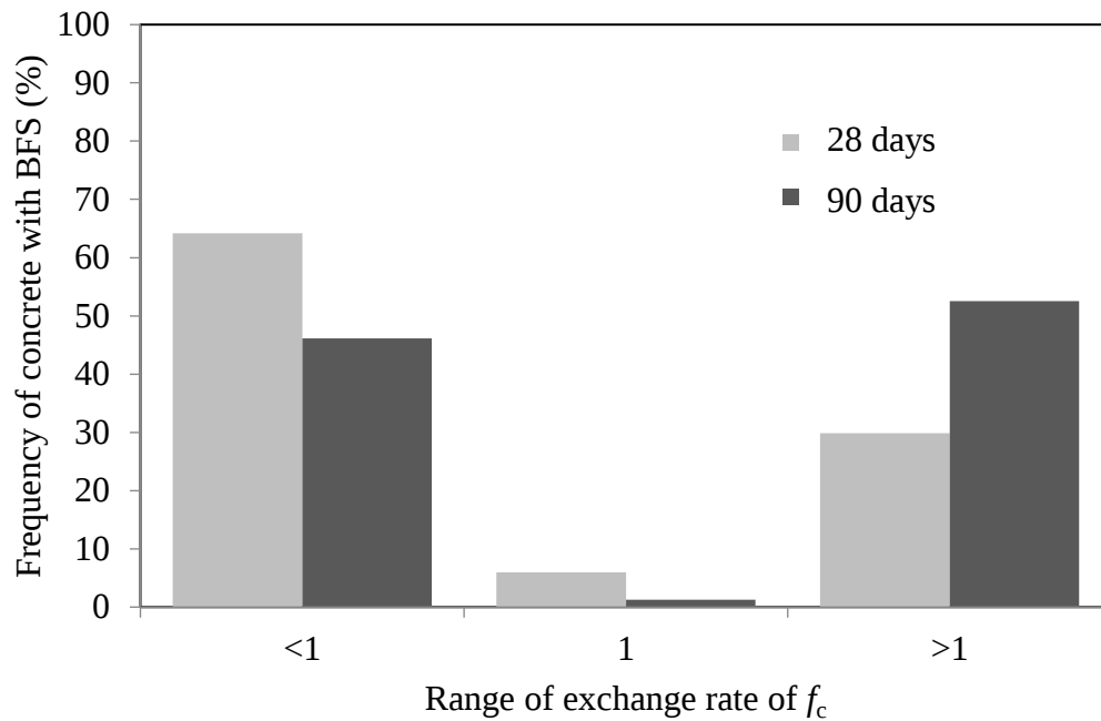
Figure 6. Frequency of the number of concrete samples with BFS related to the rate of change (efficiency) of f_c when compared to the reference concrete.
