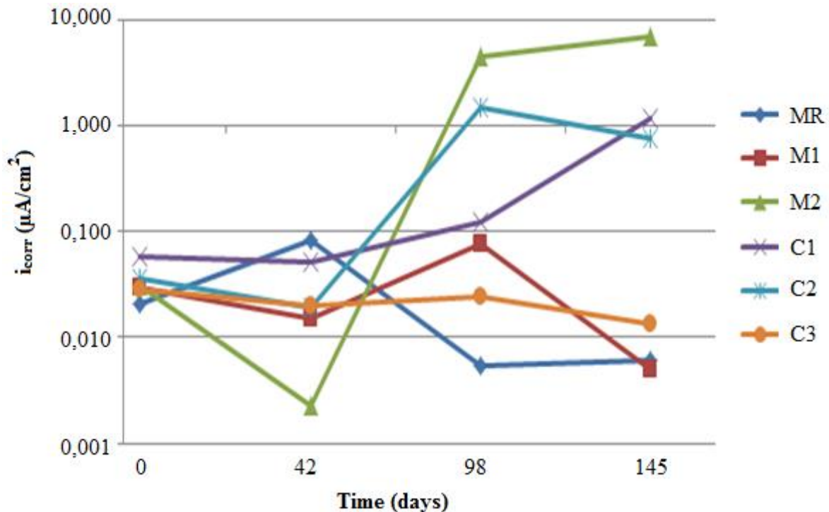
Figure 5. Corrosion rate ( i_{\text{corr}} ) in reinforcement Steel for each repair mortar.
