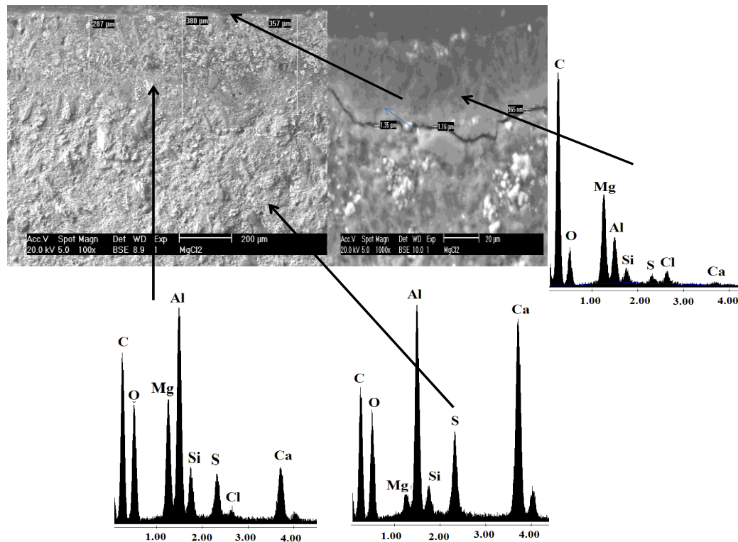
Figure 9. Micrograph of the cement after being immersed for 42 days in a \text{MgCl}_2 0.6 N solution.
