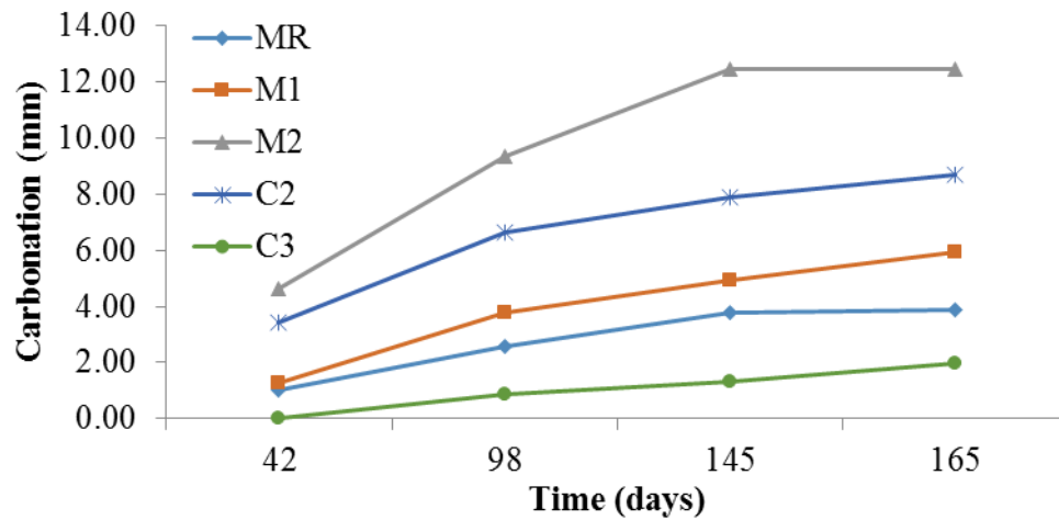
Figure 3. Carbonation Depth.
