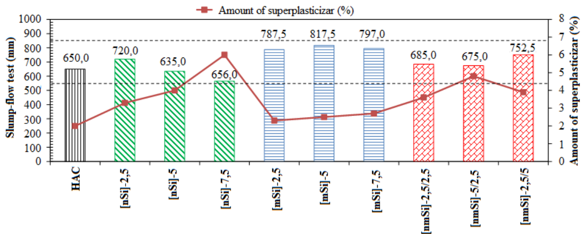
Figure 2. Slump-flow test ( d_f ) (mm) and amount of superplasticizer.
